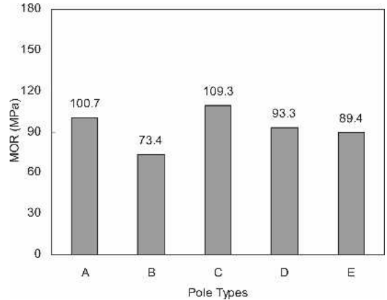
FIG. 6. Modulus of rupture of five laminated wood composite poles subjected to a cantilevered static bending. (1 MPa = 145 psi) [A] Tapered hollow member with node-like plywood webs. [B] Tapered hollow member without node-like plywood webs. [C] Tapered solid composite member. [D] Uniform-diameter hollow member with node-like plywood webs. [E] Uniform-diameter hollow member without node-like plywood webs.
