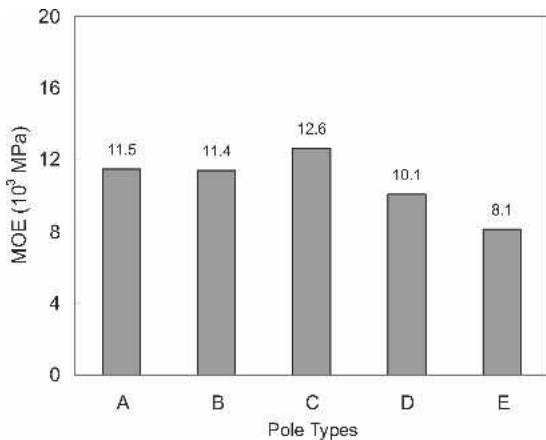
FIG. 7. Modulus of elasticity of five laminated wood composite poles subjected to a cantilevered static bending. (1 GPa = 145 \times 10^3 psi) [A] Tapered hollow member with node-like plywood webs. [B] Tapered hollow member without node-like plywood webs. [C] Tapered solid composite member. [D] Uniform-diameter hollow member with node-like plywood webs. [E] Uniform-diameter hollow member without node-like plywood webs.
