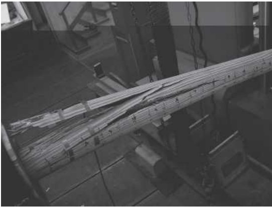
FIG. 2. The failure of a round and tapered hollow laminated composite pole with inserted node-like plywood webs when subjected to a cantilevered bending.
