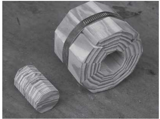
FIG. 1. A plywood-web (5.72 cm [2.25 in.] thick) and a section of the wood-laminated composite pole (diameter: 10.2 cm [4 in.]).
