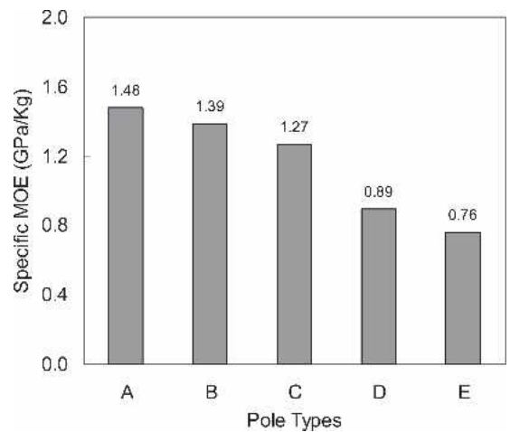
FIG. 9. Specific MOE (GPa/Kg mass) of five laminated wood composite poles subjected to a cantilevered static bending. [A] Tapered hollow member with node-like plywood webs. [B] Tapered hollow member without node-like plywood webs. [C] Tapered solid composite member. [D] Uniform-diameter hollow member with node-like plywood webs. [E] Uniform-diameter hollow member without node-like plywood webs.
