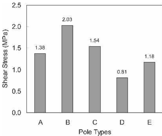
FIG. 10. Shear stress in the neutral plane at the free ends of five laminated wood composite poles when the poles failed in bending. (1 MPa = 145 psi) [A] Tapered hollow member with node-like plywood webs. [B] Tapered hollow member without node-like plywood webs. [C] Tapered solid composite member. [D] Uniform-diameter hollow member with node-like plywood webs. [E] Uniform-diameter hollow member without node-like plywood webs.
