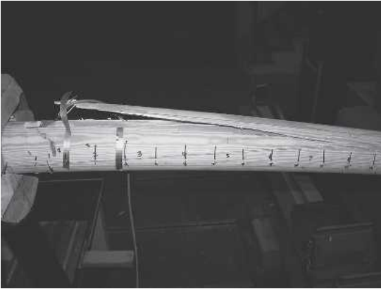
FIG. 3. The failure of a round and tapered solid wood composite pole when subjected to a cantilevered bending.
