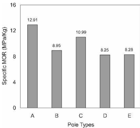
FIG. 8. Specific MOR (MPa/Kg mass) of five laminated wood composite poles subjected to a cantilevered static bending. [A] Tapered hollow member with node-like plywood webs. [B] Tapered hollow member without node-like plywood webs. [C] Tapered solid composite member. [D] Uniform-diameter hollow member with node-like plywood webs. [E] Uniform-diameter hollow member without node-like plywood webs.
