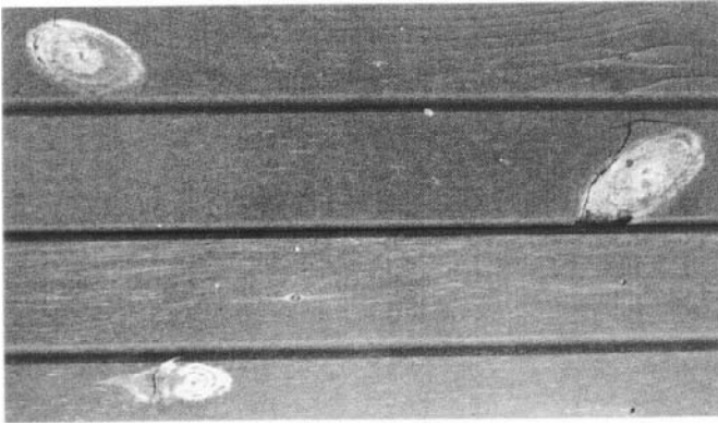
Figure 39---Exuded pitch from knots and pitch pocket on siding. (M84 0493-11)
