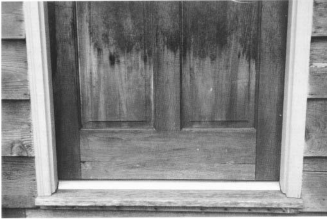
Figure 5-Rainwater splash on entrance door and siding. Rain water runs from the roof and wets the siding as it hits the concrete step.
