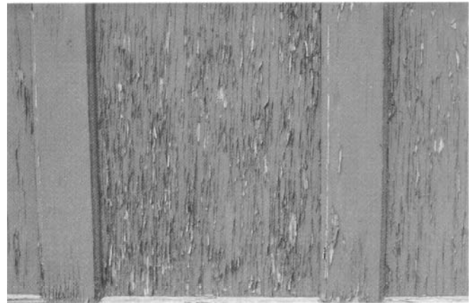
Figure 13—Early paint failure on plywood as a result of penetration of moisture into surface checks.
