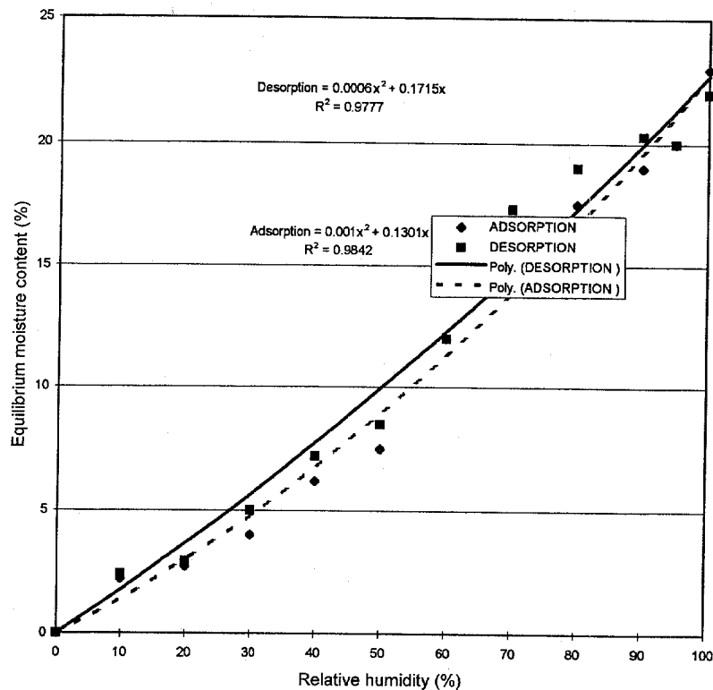
Figure 1. — Sorption curves and second order polynomial regression lines of kempas wood. Each mean value represents nine samples.
