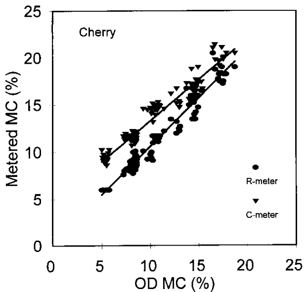
Figure 2. — Meter reading versus MC for the resistance- and capacitance-type meters for cherry wood.
