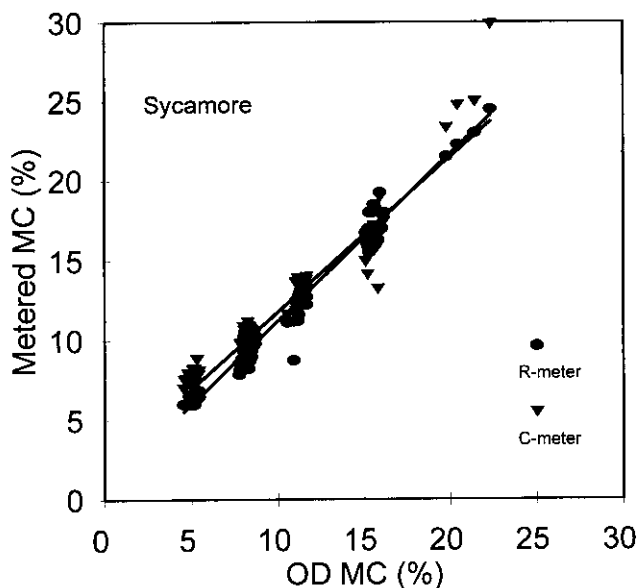
Figure 3. — Meter reading versus MC for the resistance- and capacitance-type meters for sycamore wood.
