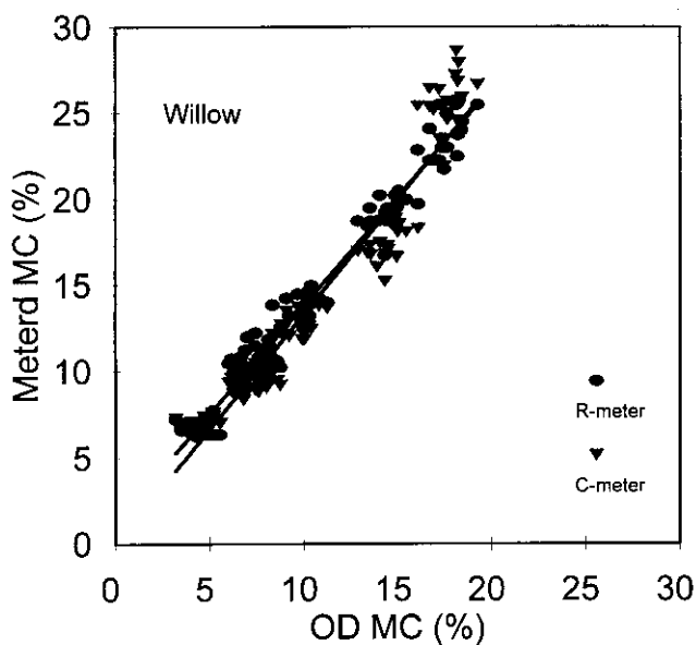
Figure 1. — Meter reading versus MC for the resistance- and capacitance-type meters for willow wood.
