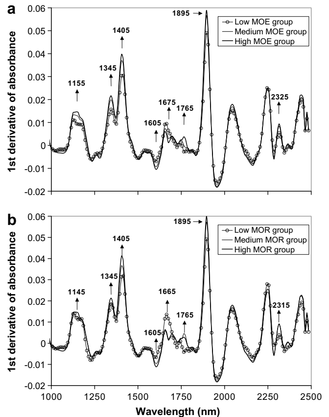
Fig. 3. The response of the first derivative of absorbance to low, medium, and high MOE (a) and MOR (b). Potential discriminatory wavelengths are labeled and marked with arrows.
