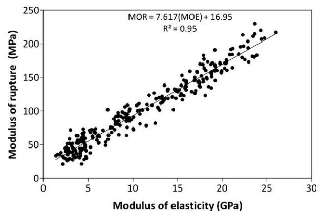
Fig. 2. The response of MOR to MOE across all ring number and heights.
