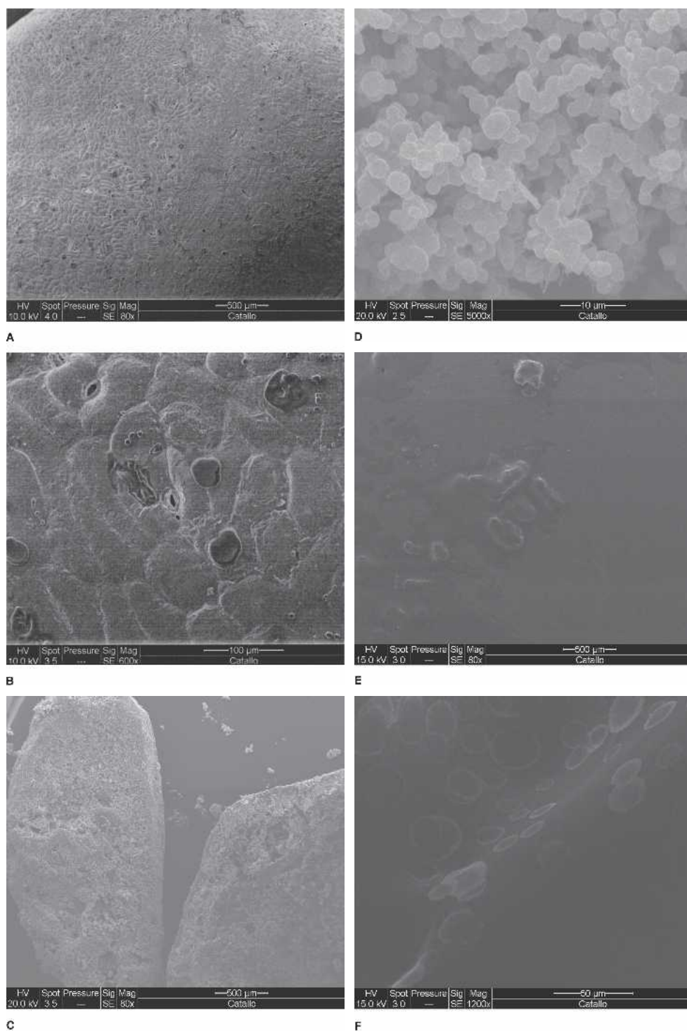
FIG. 3. Scanning electron micrographs of tallow material showing (a) control whole seed (80×), (b) control whole seed (600×), (c) HT-treated whole seed (80×), (d) HT treated whole seed (5,000×), (e) HT-treated ground seed (80×), (f) HT treated ground seed (1,200×).
