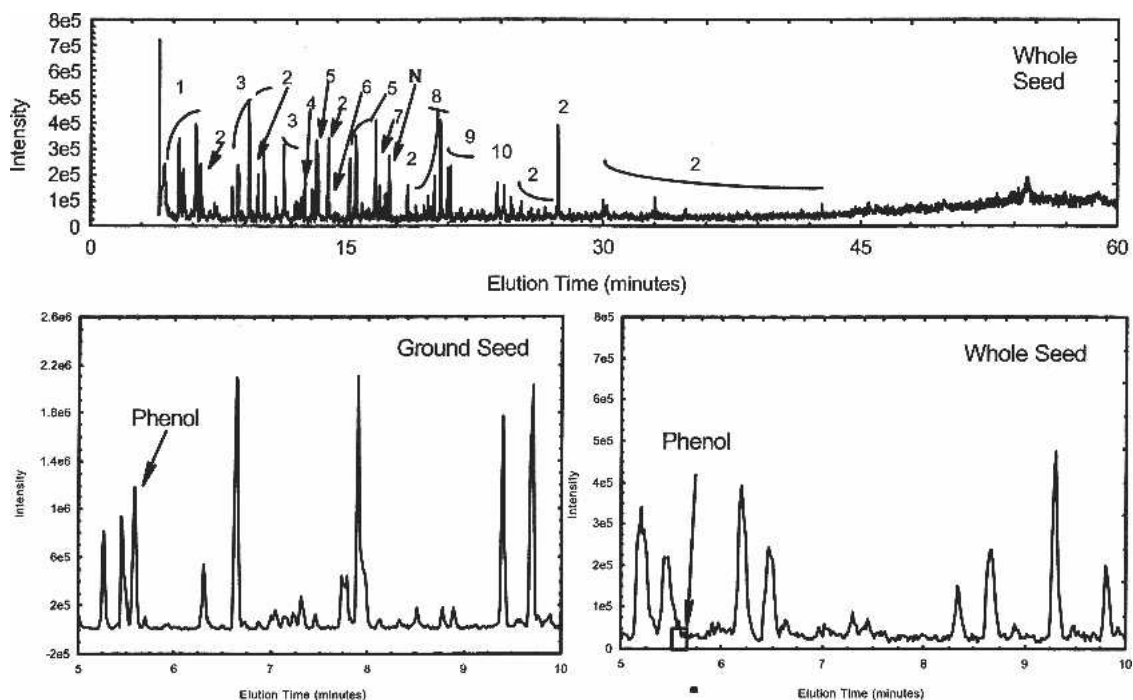
FIG. 2. Total ion chromatogram (TIC) of extracts from HT-treated (a) whole seeds; (b) and (c) showing exploded view of TIC of extracts from HT-treated ground seed and whole with respect to phenol. Compounds: 1. C_2 -Benzenes. 2. n- and branched hydrocarbons. 3. C_3 -Benzenes. 4. Indane. 5. C_1 -Indanes. 6. C_1 -Phenols. 7. C_2 -Indanes. N. Naphthalene. 8. C_5 -Benzenes. 9. C_1 -Naphthalenes. 10. C_2 -Naphthalenes.
