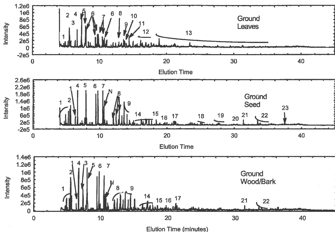
FIG. 1. Total ion chromatogram (TIC) of extracts from HT-treated (a) ground leaves, (b) ground seed, and (c) ground wood/bark. Compounds: 1. C 3 -Benzenes. 2. Phenol. 3. n-hydrocarbon. 4. Indane. 5. C 1 -Phenols. 6. C 1 -Indanes. 7. C 2 -Phenols. N = naphthalene. 8. C 2 -Indanes. 9. C 1 -Naphthalene. 10. Indole. 11. C 1 -Benzaldehyde. 12. Hydroxyindanes (6 isomers). 13. n- and branched hydrocarbons. 14. C 2 -Naphthalenes. 15. Acenaphthene. 16. C 3 -Naphthalenes. 17. C 1 -Fluorene. 18. Anthracene/Phenanthrene. 19. C 1 -Anthracenes/Phenanthrenes. 20. Fluoranthene. 21. Pyrene. 22. mass 216, e.g., C 1 -Pyrenes and benzofluorenes. 23. mass 228, e.g., Triphenylene, Benzanthracene, Chrysene.
