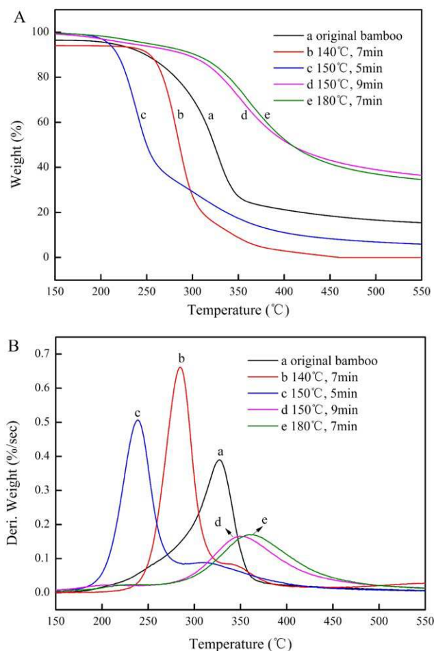
Figure 5. TG (A) and DTG (B) curves for (a) original bamboo, decomposed residues (b) 140 °C, 7 min, (c) 150 °C, 5 min, recondensed residues (d) 150 °C, 9 min, (e) 180 °C, 7 min. Other conditions: glycerol/methanol, 2/1; microwave power, 550 W; sulfuric acid, 1.75%; solvent/bamboo, 4/1. [Color figure can be viewed in the online issue, which is available at wileyonlinelibrary.com .]
