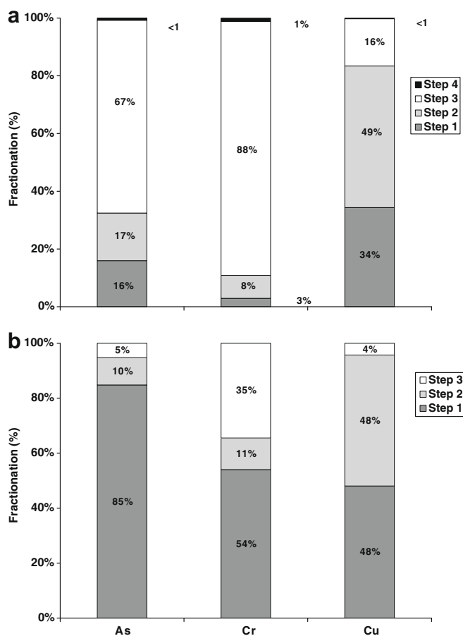
Fig. 2. Distribution of three elements in (a) original CCA-treated wood particles and (b) liquefied CCA-treated wood sludge among each fraction from the sequential extraction.
