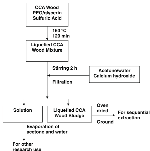
Fig. 1. Flowchart of liquefaction of CCA-treated wood and precipitation for liquefied CCA-treated wood sludge.
