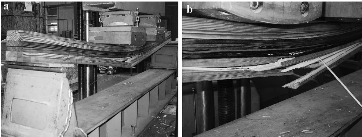
Figure 2.—Bending tests of laminated crossarms made of decommissioned chromated copper arsenate-treated utility pole wood: (a) a laminated beam (Composition C) was tested in two-point loading and (b) failure detail of a laminated crossarm after the bending test.
