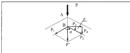
FIG. 6. Load vectors applied to the small-scale composite poles in a crushing test.
