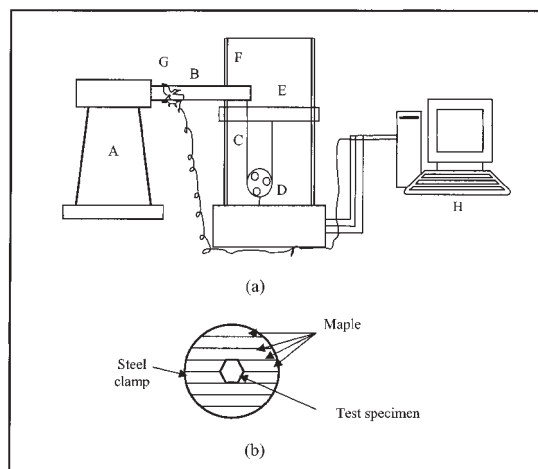
FIG. 3. A schematic diagram of the flexural testing device.
