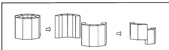
FIG. 4. A schematic diagram of a sample cutting plan for the glue-line shear test.
