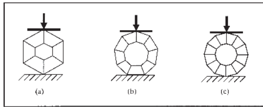
FIG. 5. Crushing test set-ups for wood laminated composite poles with 6 (a), 9 (b), and 12 (c) sides.
