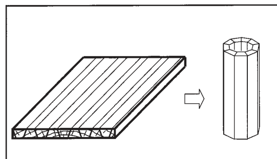
FIG. 2. A schematic diagram of a strip-cutting plan for a nine-strip composite pole.
