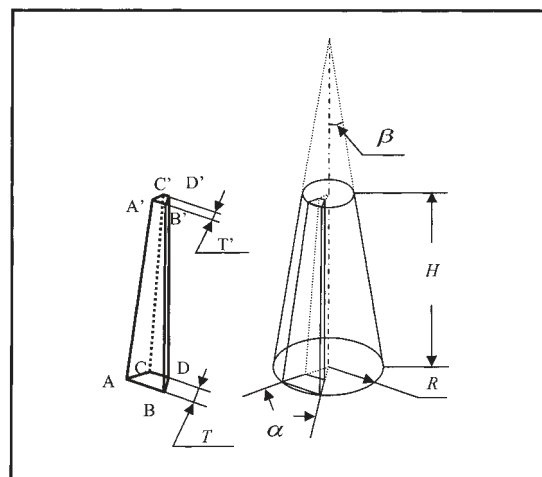
FIG. 1. A schematic diagram of a wood strip composite pole and one of its strips.
