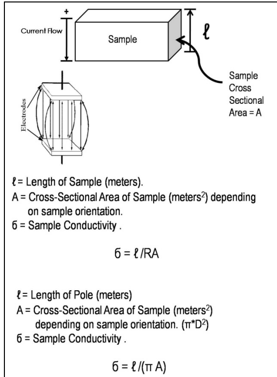
Figure 4. Measurements were made across the longitudinal face (12 mm, ℓ) and in the radial direction across the grain (16 mm, ℓ) as seen above, and Siemens per meter were calculated for wafers and poles.
