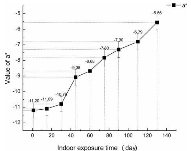
Figure 6.—Changes in a^* values of treated Neosinocalamus affinis bamboo samples with respect to indoor exposure time.
