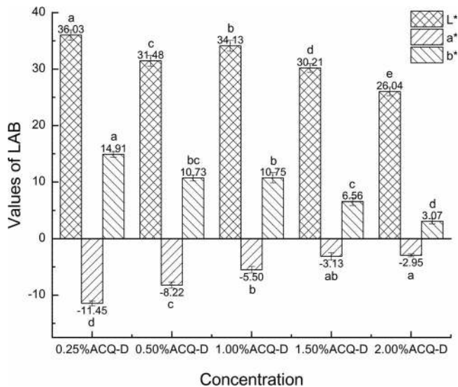
Figure 4.—Effect of alkaline copper quaternary type D (ACQ-D) concentration on the color parameters of Neosinocalamus affinis bamboo; lowercase letters mean significant differences (at the 0.05 level) of L^* a^* b^* values with different ACQ-D concentrations.
