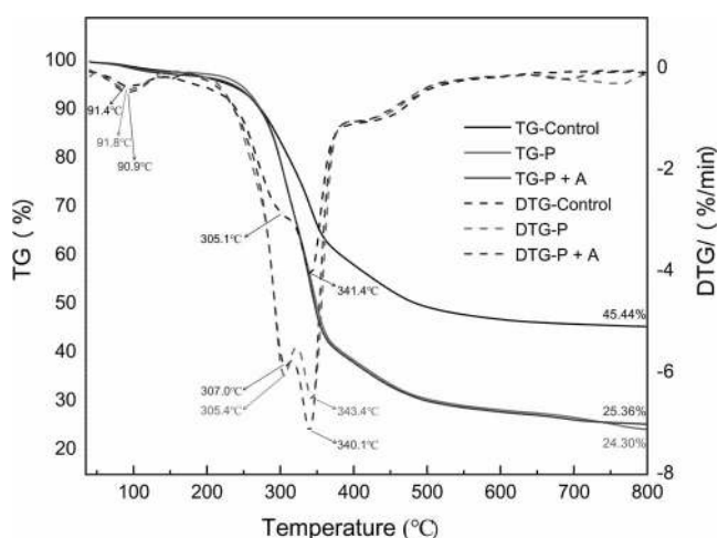
Figure 8.—Thermogravimetric/derivative thermogravimetric (TG/DTG) curves of the green surface of the control, pretreated (P), and treated (P + A) samples of Neosinocalamus affinis .
