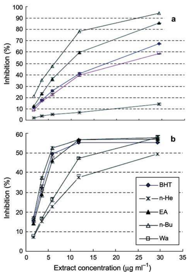
Figure 1 (a) DPPH• and (b) ABTS• + scavenging capability of bark extracts of Port-Orford cedar. Note: n-He, EA, n-Bu and Wa indicate bark extracts fractionated in n -hexane, ethyl acetate, n -butanol, and deionized water, respectively. Each value is the mean \pm SD of three measurements. Some of the SD values are too small to show.
