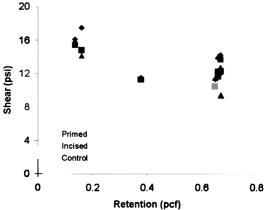
Fig. 6. Effects of CCA retention on the bonding shear strength of laminates made from decommissioned CCA-treated utility poles.
