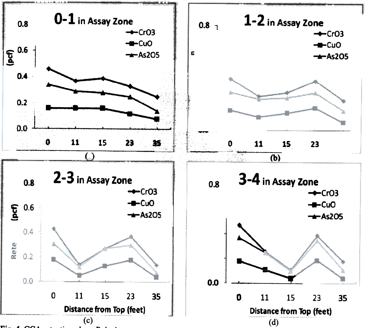
Fig. 4. CCA retention along Pole 4.
